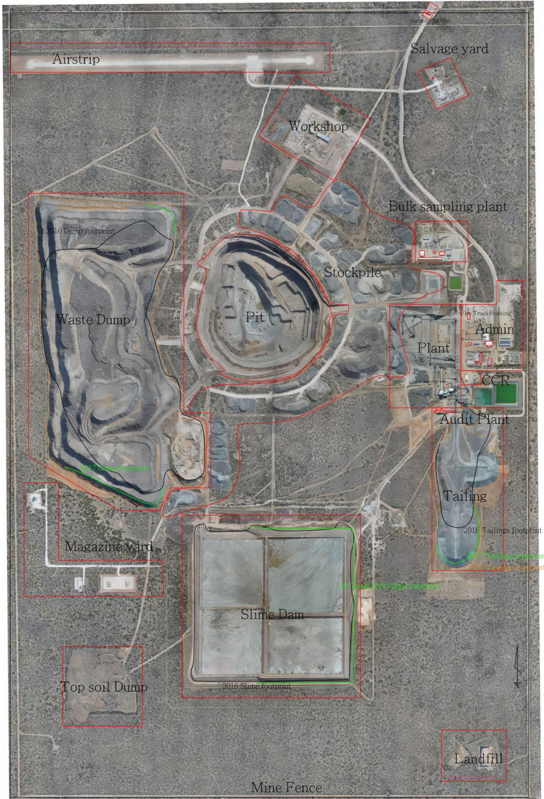
Figure 1: The Karowe Diamond Mine and existing infrastructure (2018)
