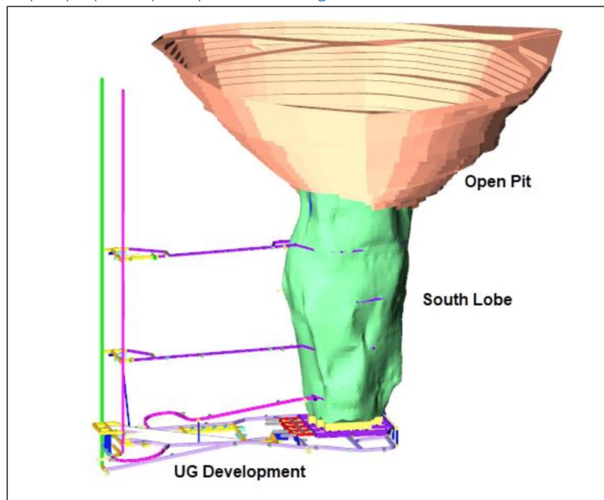
Figure 2: KDM's open pit (brown) and planned underground mine
