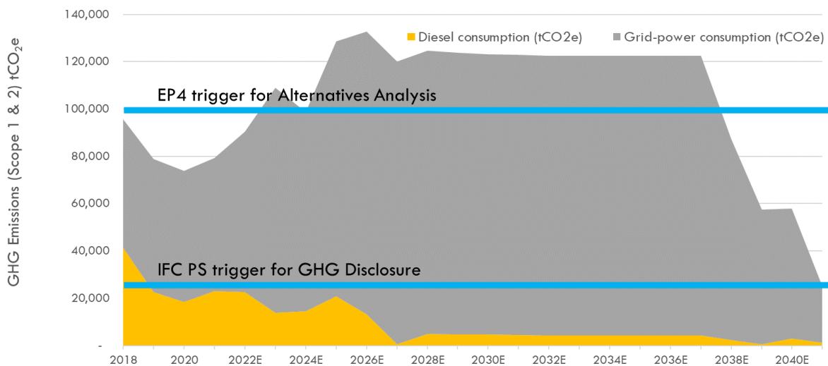
Figure 9: The Project’s estimated GHG emission profile
